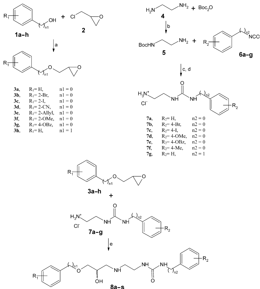
Scheme 2. Synthesis of the \beta_1 -AR ligands 8a-s . Reagents: (a) 2N NaOH or Na, toluene for compound 3h ; (b) CH 2 Cl 2 ; (c) Et 2 O or THF; (d) HCl, MeOH; (e) 10N NaOH, n -PrOH, H 2 O.
