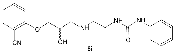
Scheme 1. Lead structure of ICI 89,406 8i .
