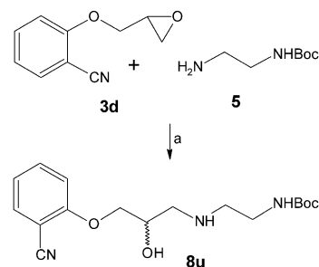
Scheme 4. Synthesis of the \beta_1 -AR ligand 8u . Reagents: (a) n -PrOH.
